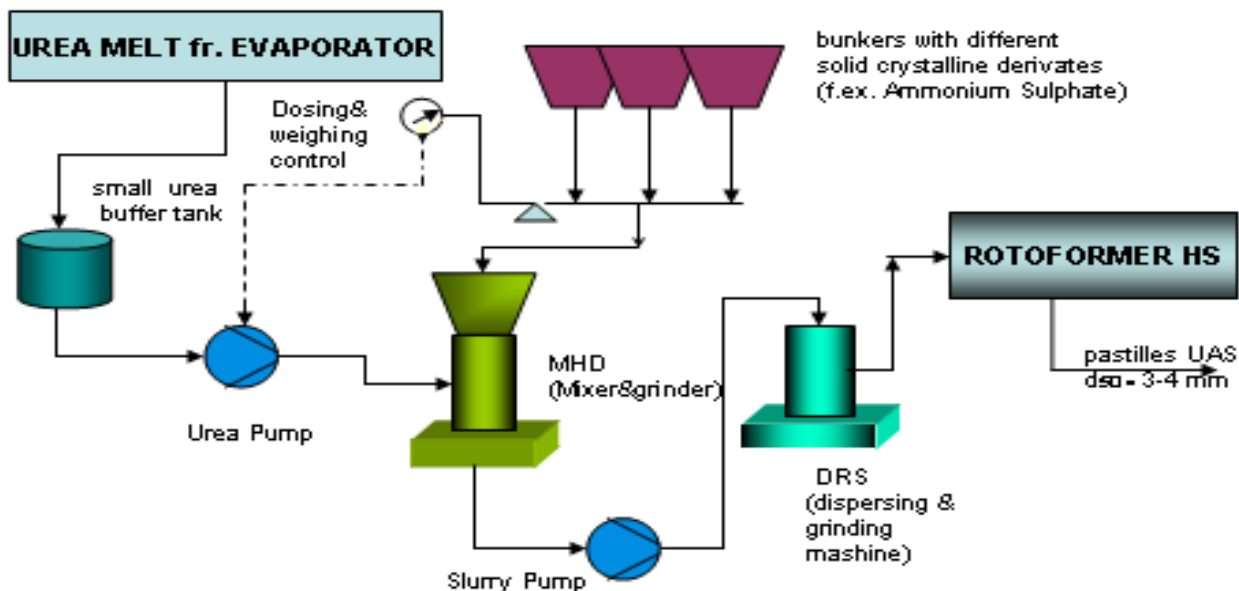
Sketch of mixing and grinding preparation
